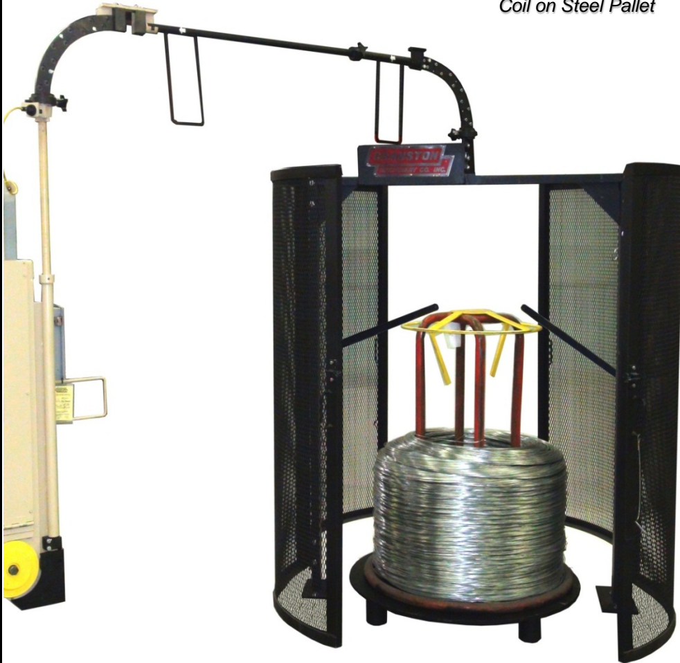
Fixed Position Cage Coil on Steel Pallet
